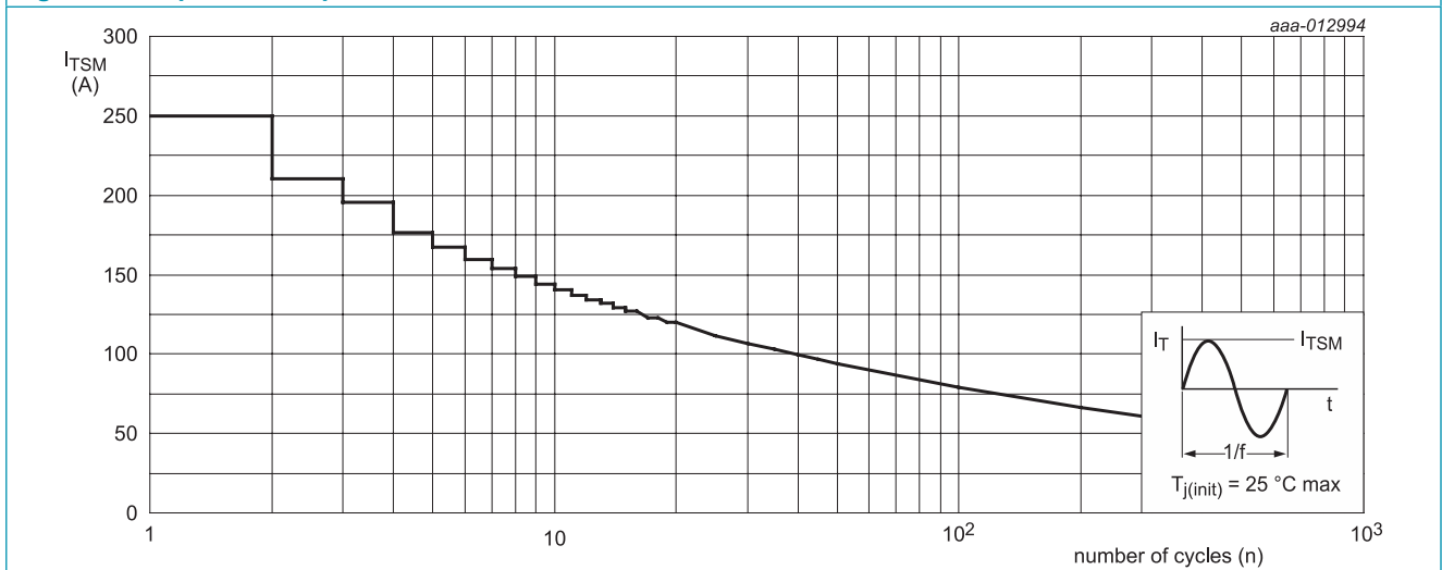
f = 50 Hz Fig. 4. Non-repetitive peak on-state current as a function of the number of sinusoidal current cycles; maximum values
