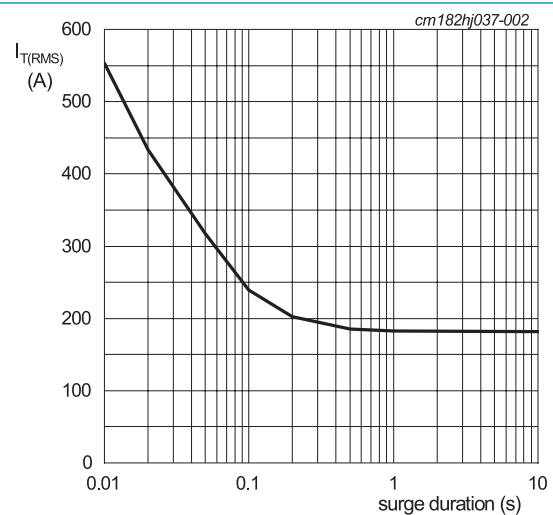
Fig. 2. RMS on-state current as a function of surge duration; maximum values f = 50\text{ Hz} ; T_{mb} = 107\text{ °C}
