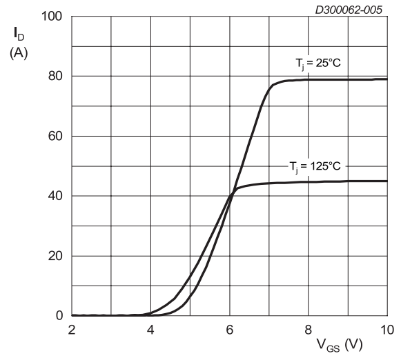
Fig. 5. Drain current as a function of gate-source voltage; typical values V_{DS} = 20 V
