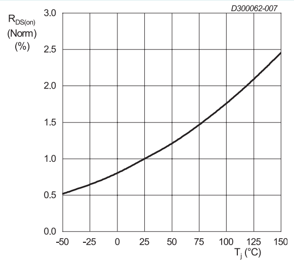
Fig. 7. Normalized drain-source on-state resistance as a function of junction temperature V_{GS} = 10 V; I_D = 15 A
